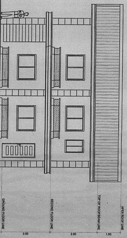
FRONT ELEVATION SCALE: 1 : 50 MTS.
