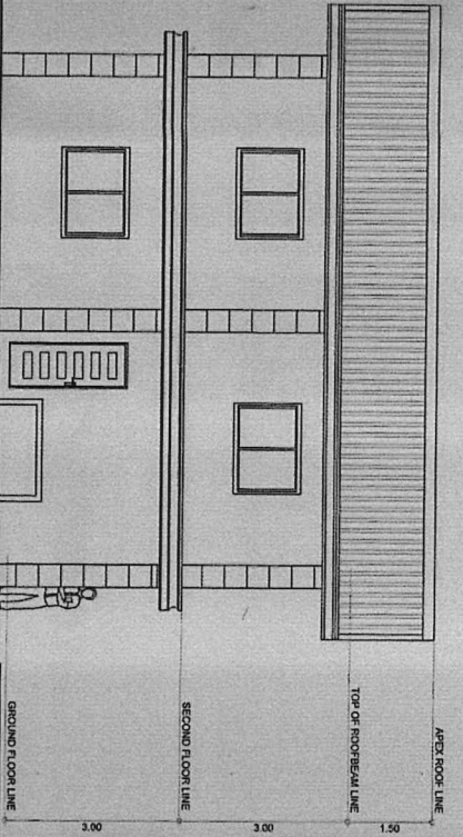
REAR ELEVATION SCALE: 1 : 50 MTS.
